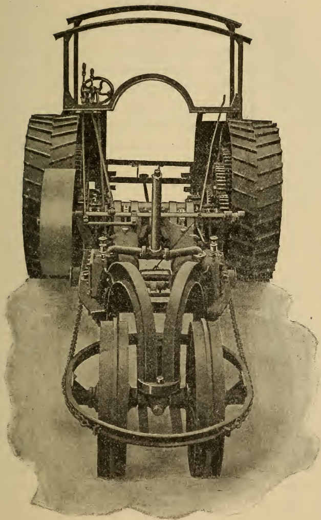
FIG. 27.—FRONT VIEW—WITHOUT BOILER—OF THE AULTMAN TRACTION ENGINE.
